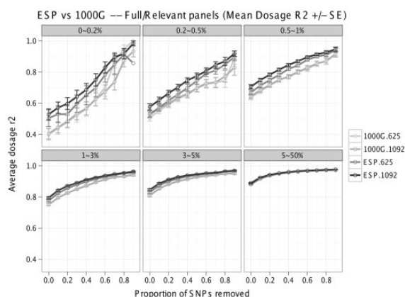
Fig. 2. Comparison of dosage r^2 between ESP and 1000G full/relevant panel imputation. The x -axis is the proportion of SNPs that were removed based on elevated R_{sq} threshold (QC). The y -axis is the mean dosage r^2 (squared Pearson correlation between imputed dosages and experimental genotypes)
