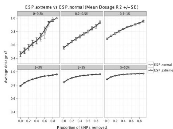
Fig. 3. Comparison of dosage r^2 between ESP.extreme and ESP.normal imputation. The x -axis is the proportion of SNPs that were removed based on elevated R_{sq} threshold (QC). The y -axis is the mean dosage r^2 (squared Pearson correlation between imputed dosages and experimental genotypes)
